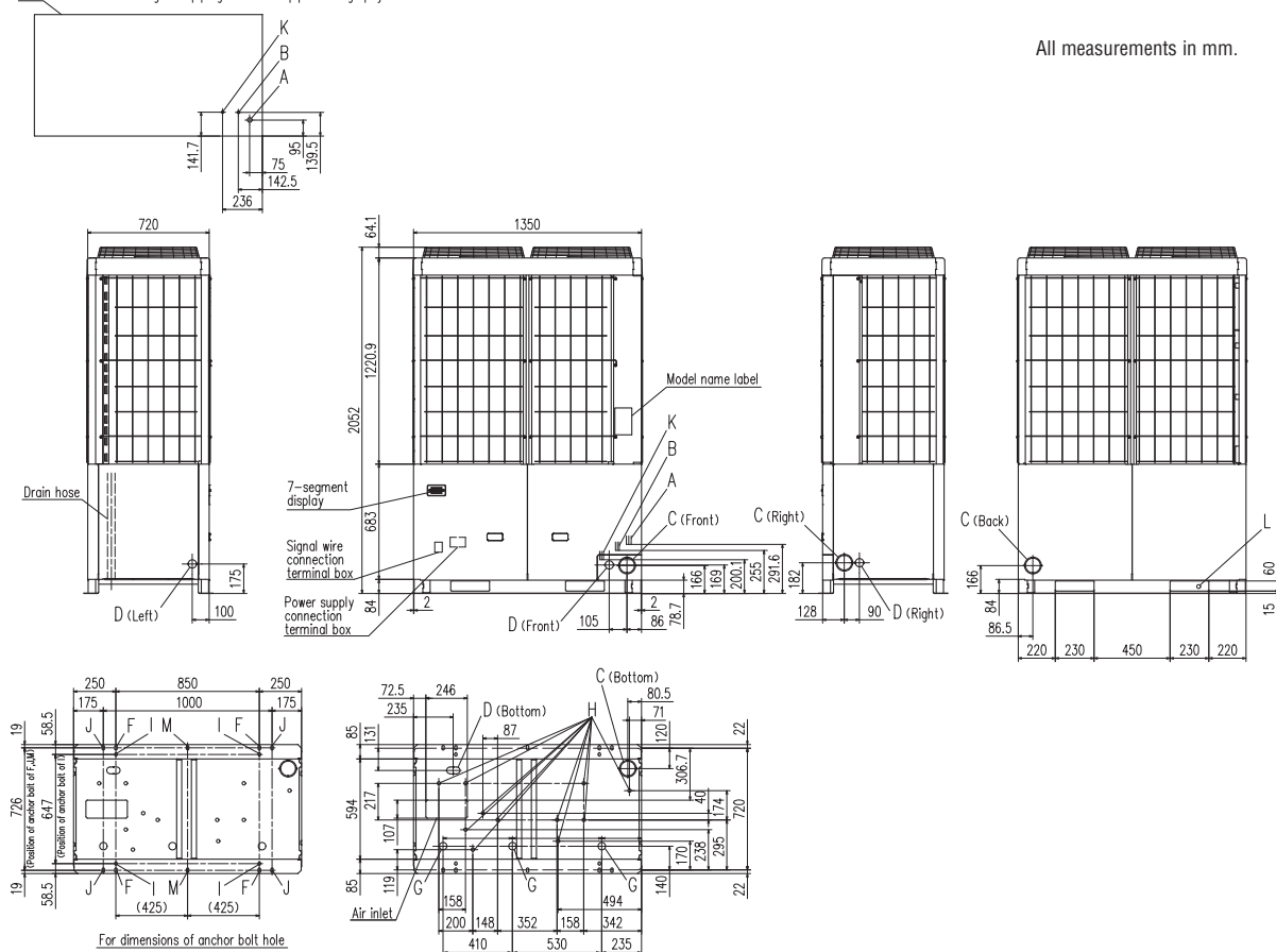
Back Dimensions of refrigerant piping connection pipe (ichnography)
