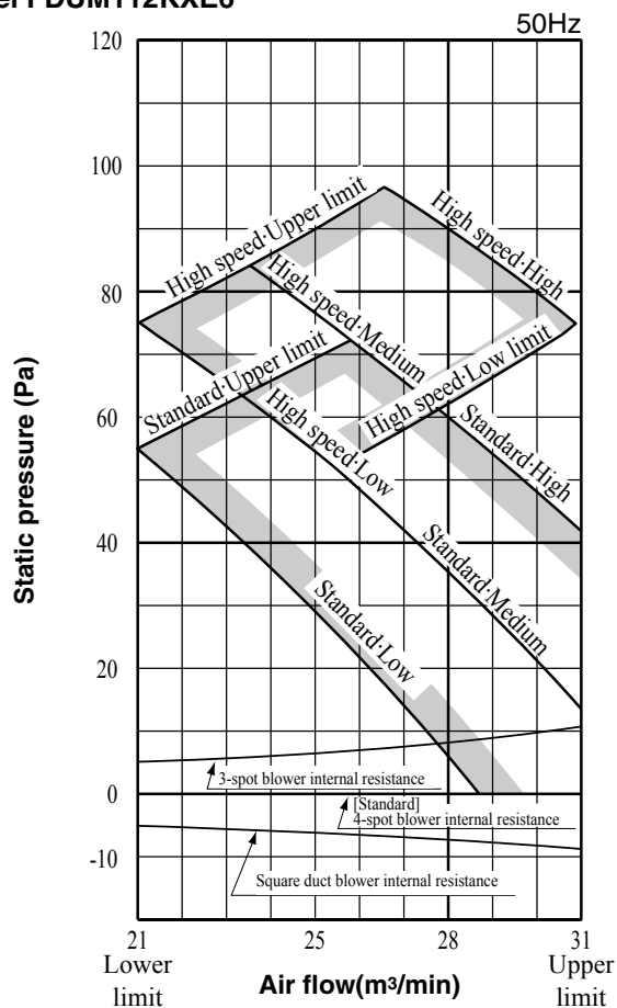
Model FDUM112KXE6
