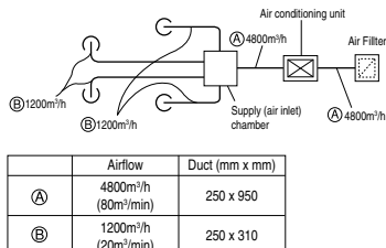
(Simplified duct dimension selection table)
