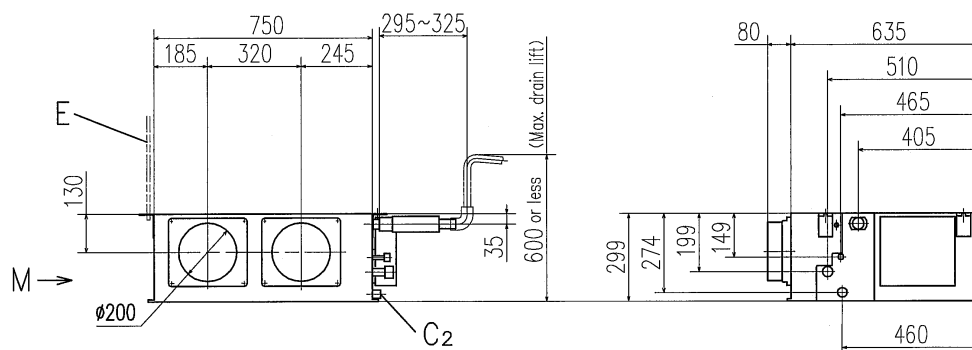
View M
