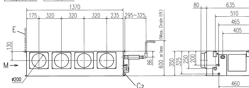
View M
