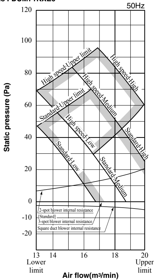
Models FDUM71KXE6
