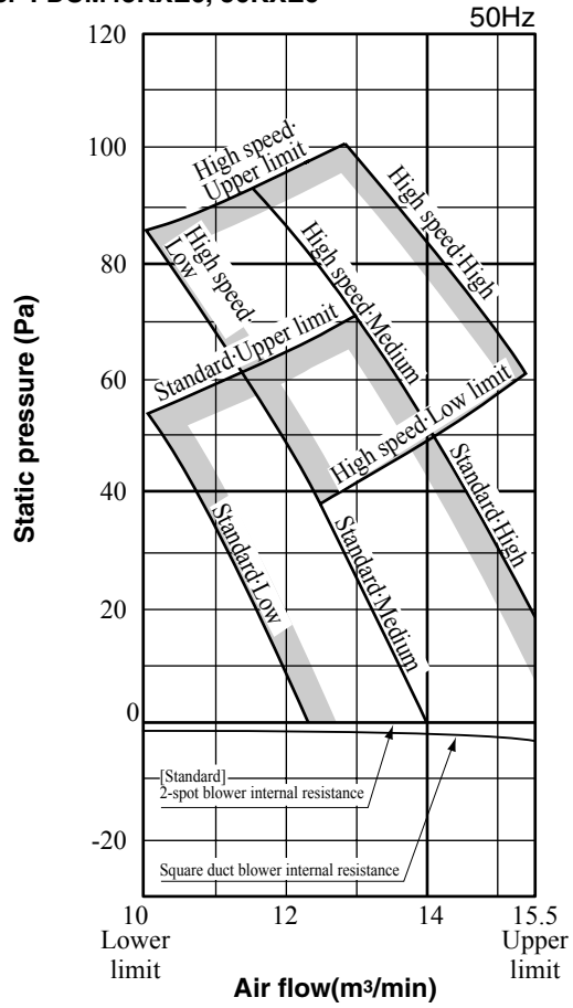
Models FDUM71KXE6
